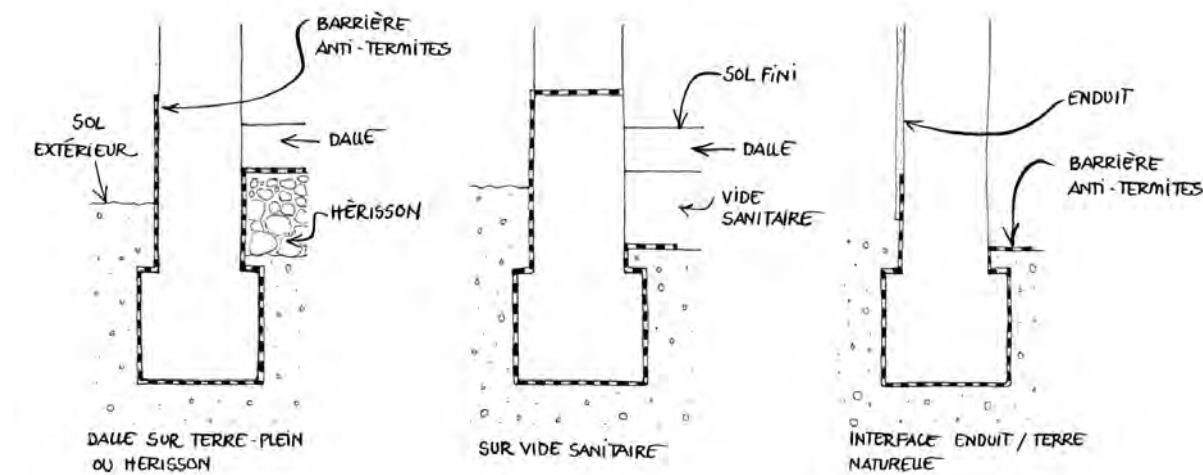
Figure 6: Barrière anti-termites
